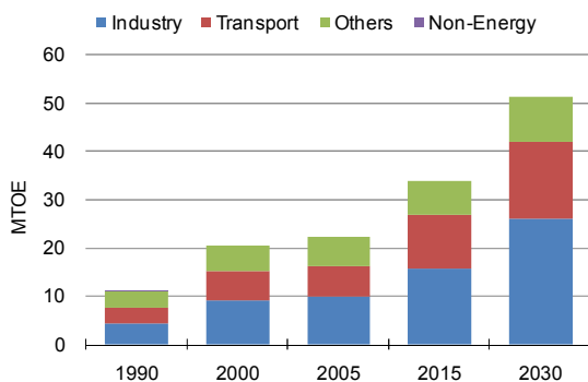
Figure CHL2: Final energy demand
