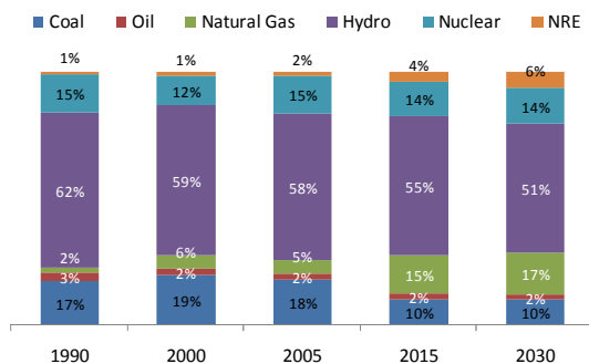
Figure CDA4: Electricity generation mix
