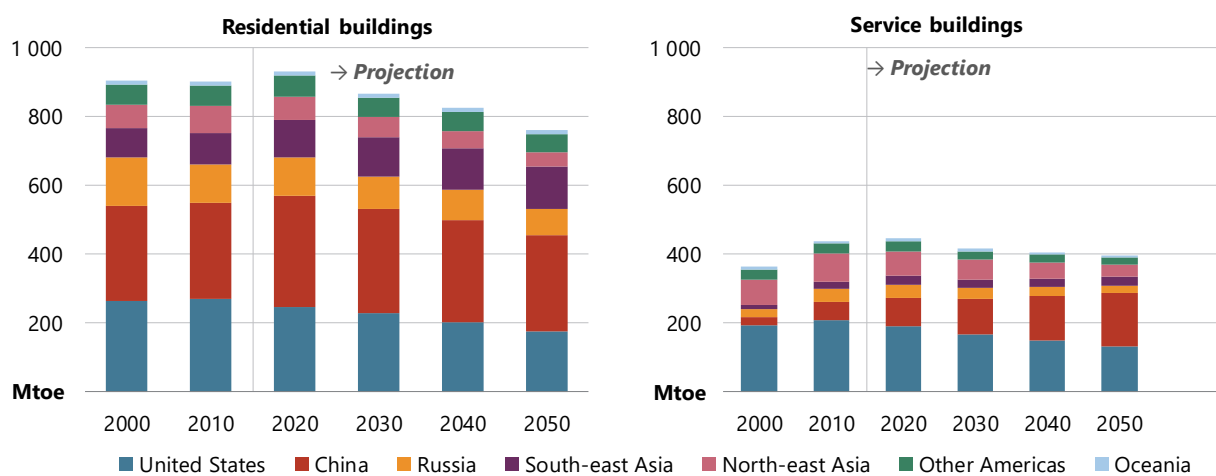
Figure 6.13 • 2DC: Buildings final energy demand by region, 2000-50
